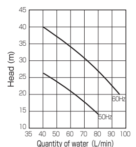
PEC900B1-VW
