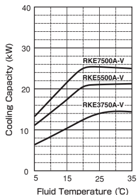
RKE3750 / 5500 / 7500A-V
