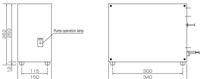
Cooling unit
