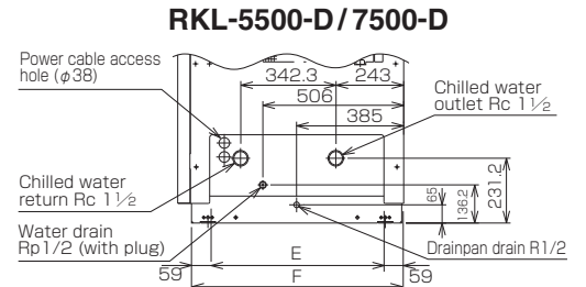
Water piping plate detail
