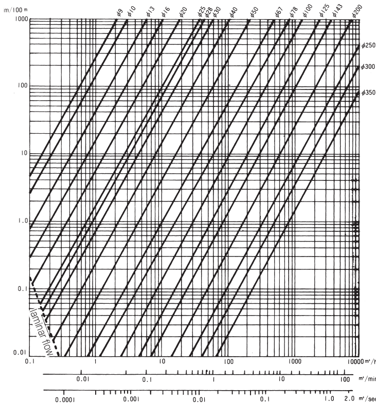
Head Loss within Hard PVC Pipe
