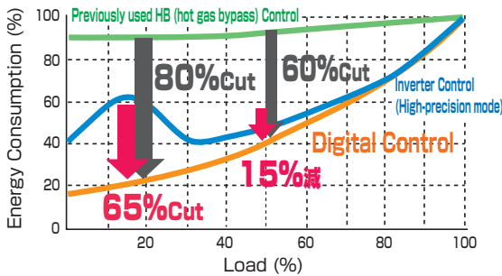
Comparison of Energy Savings by Control Method
