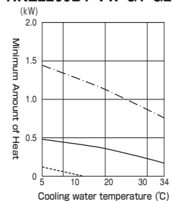
RKE2200B1-VW-G1·G2
