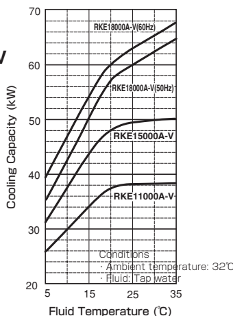
RKE11000 15000 18000A-V
