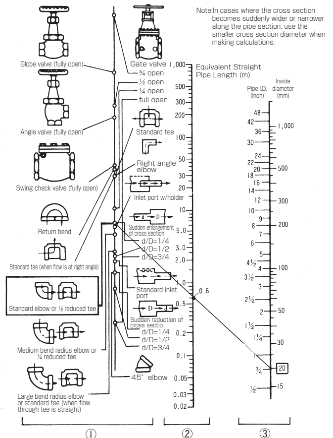
Equivalent Lengths for Valves and Couplings
