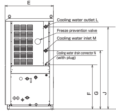
Water piping plate detail
