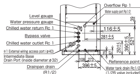
Water piping plate detail
