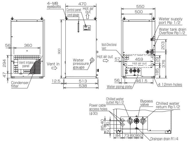
Water plumbing plate is detailed
