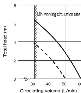
RKS1500F
