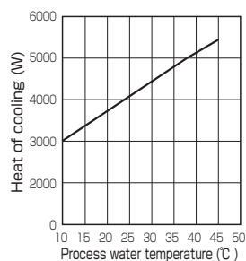
PEC900B1-VW
